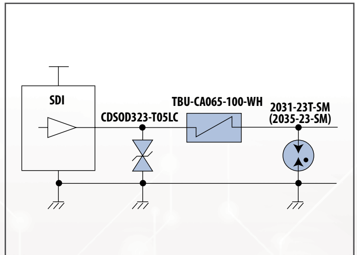
Figure 6 Video Surveillance
