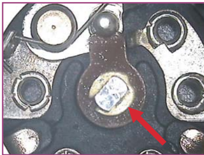
Old design with c-clip
