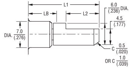
FLATTED SHAFT
