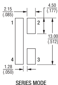
SERIES MODE
