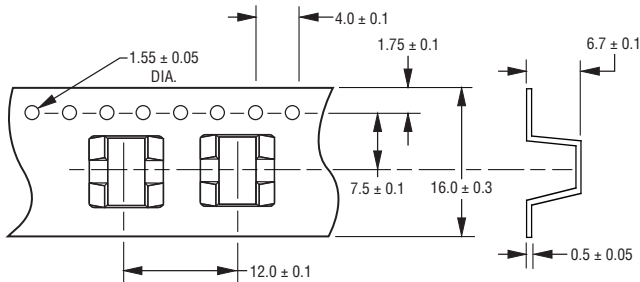
DIMENSIONS: MILLIMETERS
