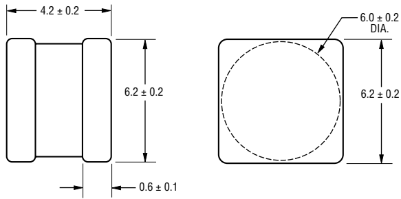
DIMENSIONS: MILLIMETERS
