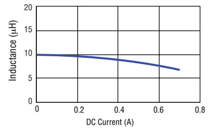
SRN2508A-100M
