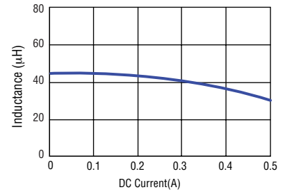
SRN3015TA-470M
