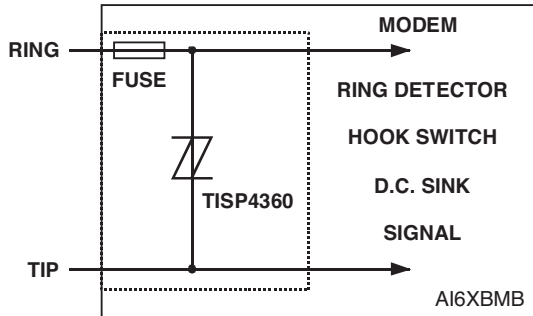
Figure 16. Modem Inter-wire Protection
