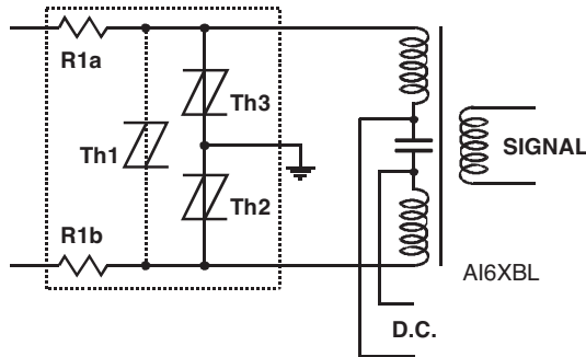
Figure 18. ISDN Protection
