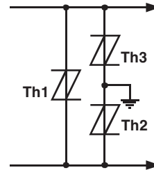
Figure 12. Multi-point Protection
