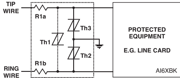
Figure 17. Protection Module
