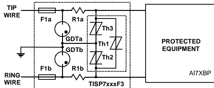
Figure 36. Protection Module
