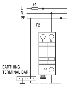
2P (2+0) for single phase (TT/TN)
