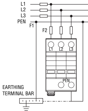
3P (3+0) for 3 phases (TN-C/IT)
