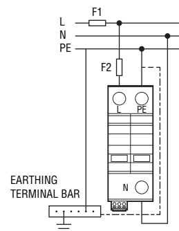
2P (1+1) for single phase (TT/TN)
