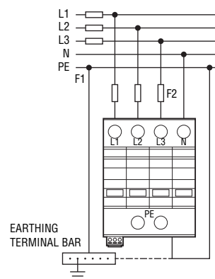
4P (3+1) for 3 phases (TT/TN)
