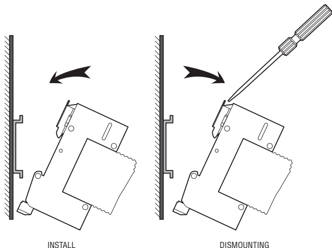
Fig.1: SPD mounting on DIN-Rail
