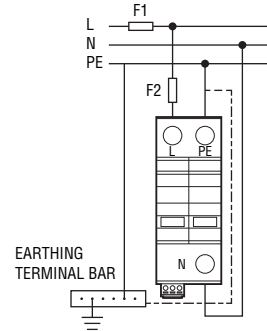
2P (1+1) for single phase (TT/TN)
