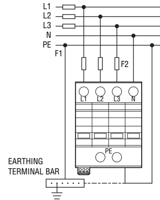
4P (3+1) for 3 phases (TT/TN)
