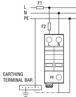
2P (2+0) for single phase (TT/TN)
