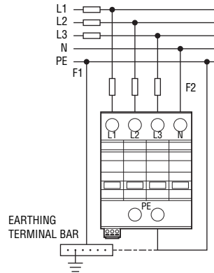
4P (4+0) for 3 phases (TT/TN)
