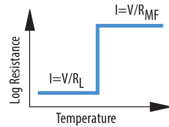
PTC Response Characteristic
