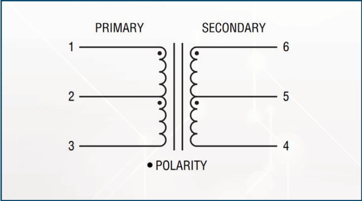
Schematic 1
