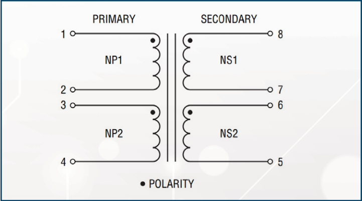
Schematic 2
