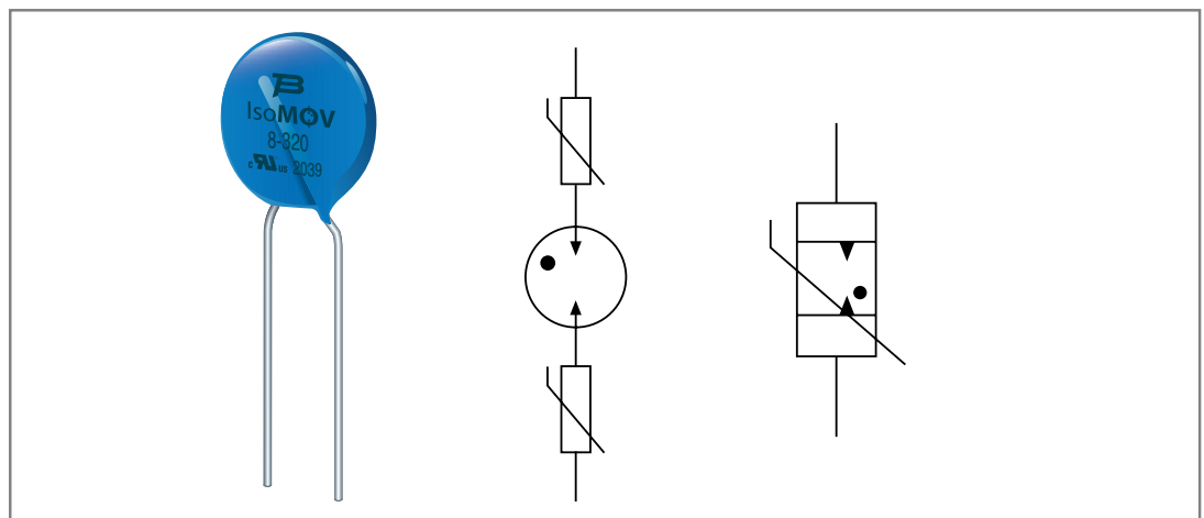
Figure 1 - The fully integrated IsoMOV™ protector offers a robust, space-saving design.
